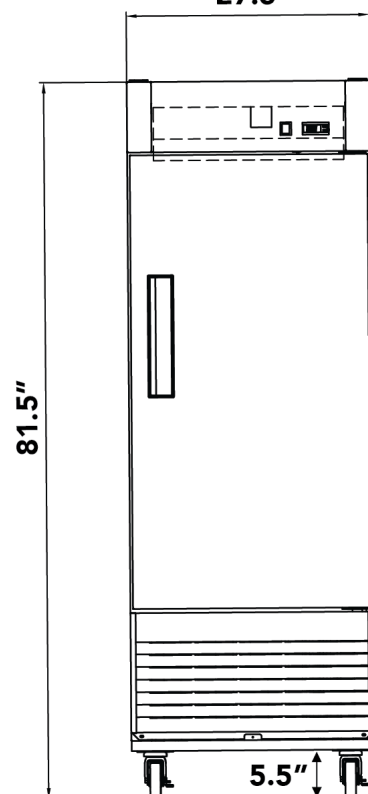
FRONT VIEW 27.5"
